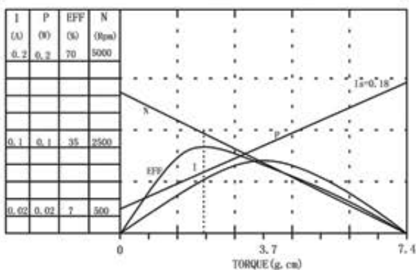
FF-030PA-08250 2.5VDC
