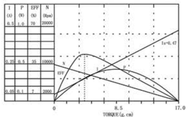
FF-030PA-09210 4.7VDC
